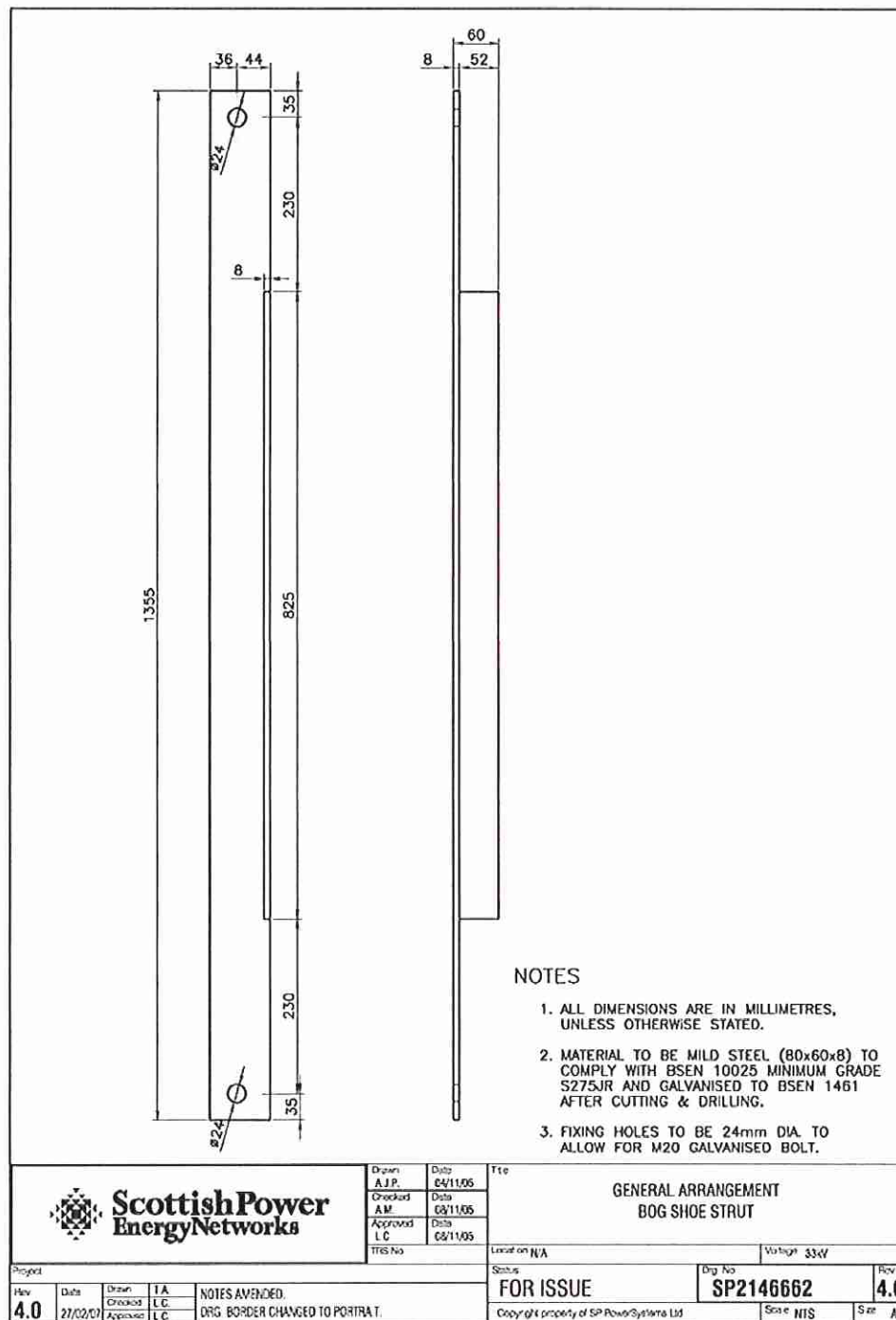
Figure 55 General Arrangement Bog Shoe Strut (Drawing SP2146662)
